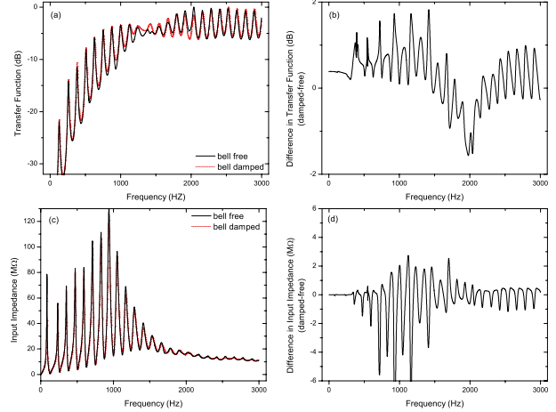
Fig 2 : (a) Predicted transfer function of trumpet with walls free to vibrate (black, solid) and with the walls heavily damped (red, dashed). (b) Difference in the theoretical transfer functions. (c) Predicted input impedance of trumpet with walls free to vibrate (black, solid) and with the vibrations heavily damped (red dashed). (d) Difference in the theoretical input impedance.
