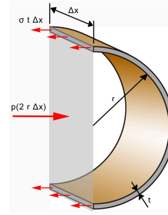
Fig 1 : Wall forces caused by internal pressure
